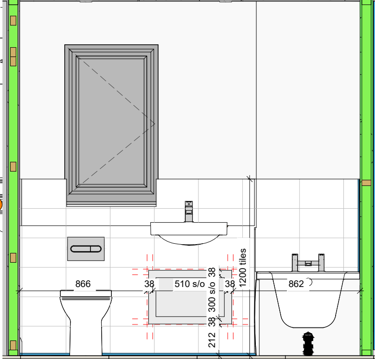
A Bathroom - View A 1 : 25
