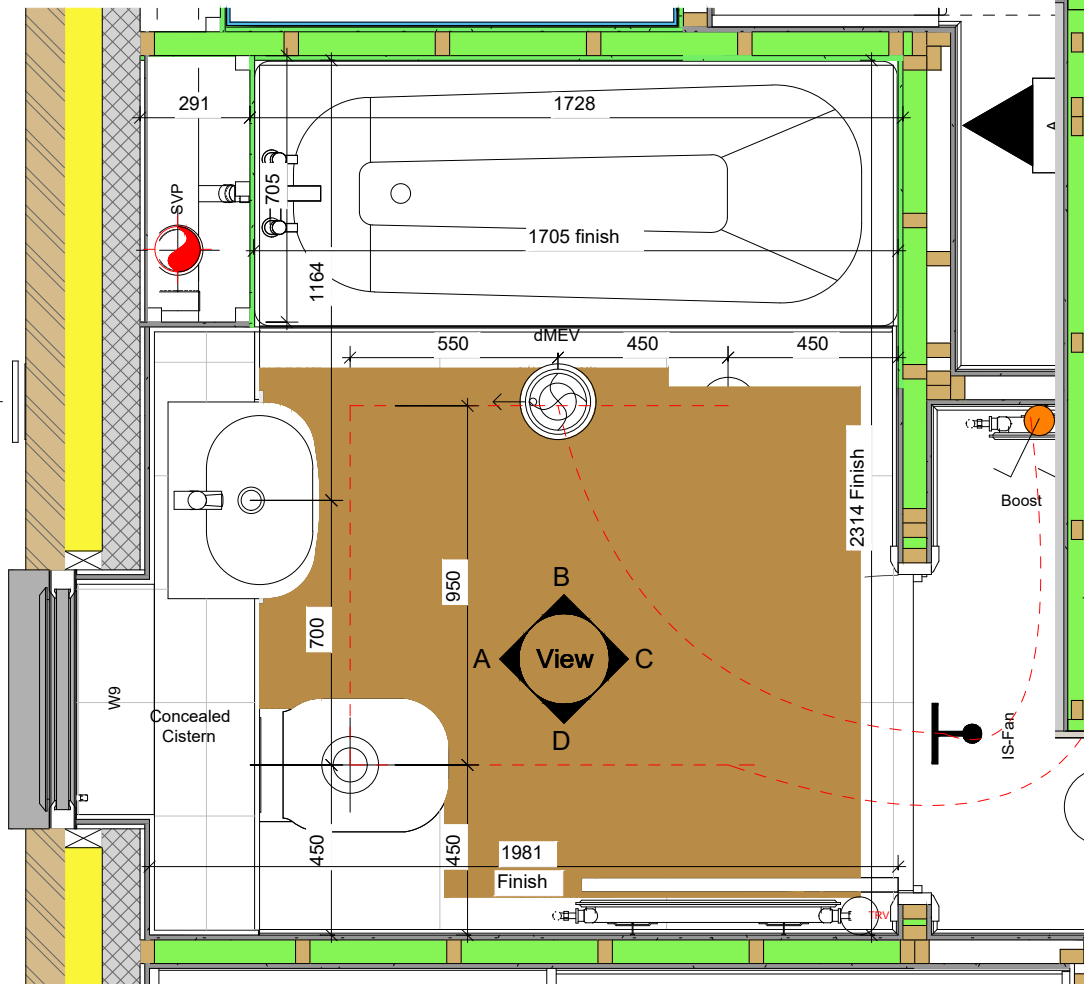
1 Bathroom Layout 1 : 20
